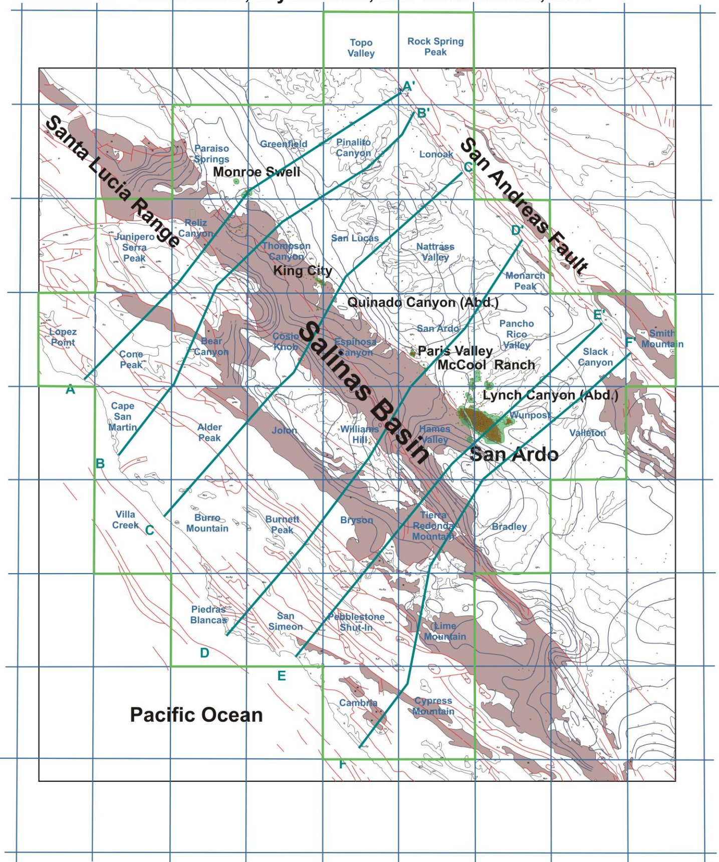
Map showing study cross section lines, 7.5' USGS quads. used in study, distribution of Monterey Formation surface exposures (fills), gravity contours, and surface geology.
