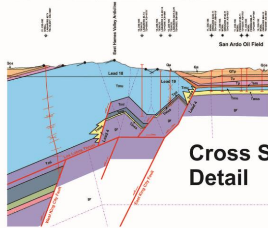
Salinas Basin Cross Section
